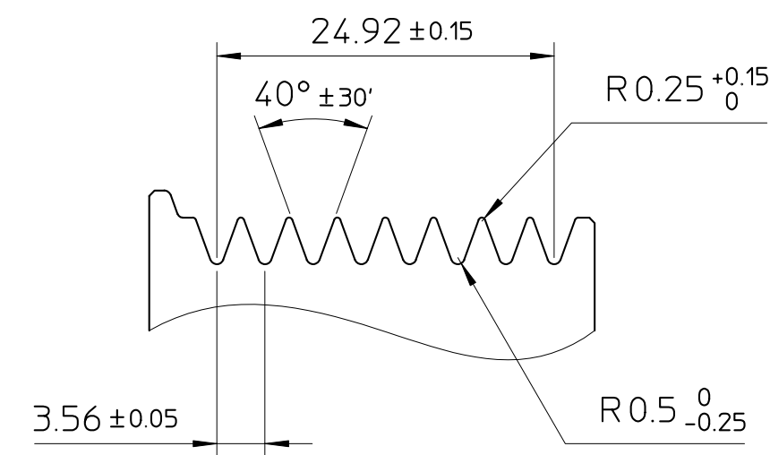
DETAIL OF ROTOR GROOVE(2:1)
