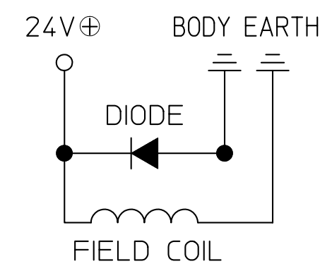
CIRCUIT DIAGRAM
